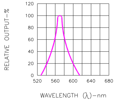
Fig.2 SPECTRAL RESPONSE
